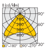
Wide 90°
