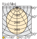
Diffus - Wide 60°
