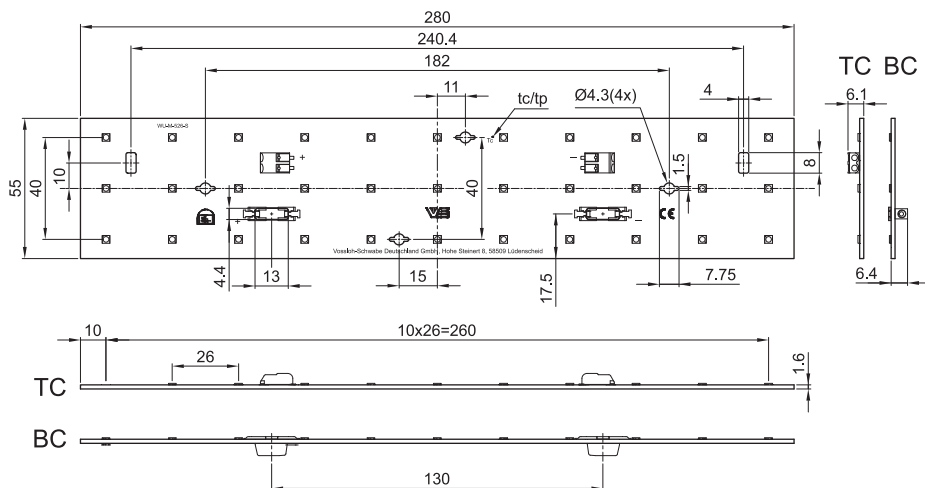
WU-M-526-S-TC/-BC
