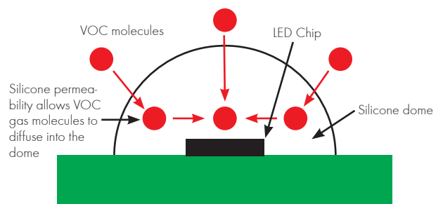
Figure 1: Permeability of the LED's potting agent to gaseous components due to the high porosity of cured silicones
