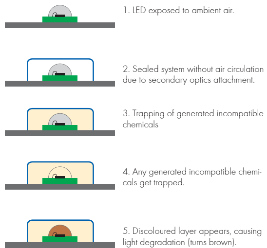
Figure 5: Schematic of an LED displaying the discolouration effect, caused by incompatible chemicals due to airtight operating conditions.
